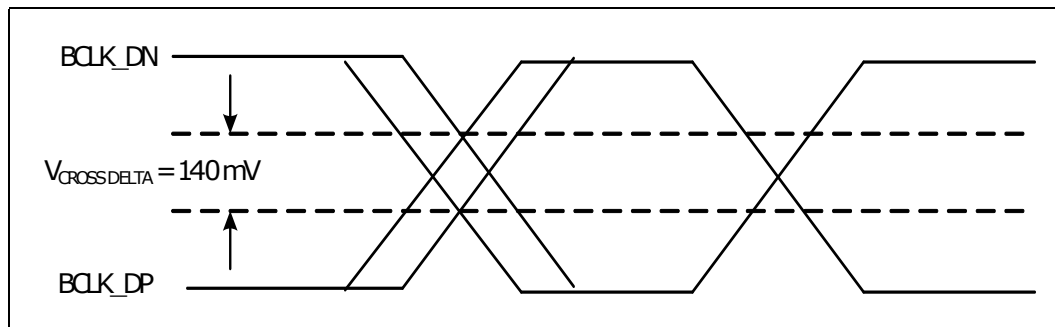
Figure 7-9. BCLK{0/1} Single Ended Clock Measurement Points for Delta Cross Point
