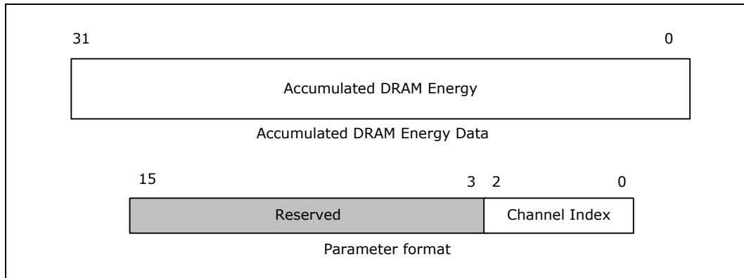
Figure 2-17. Accumulated DRAM Energy Data
